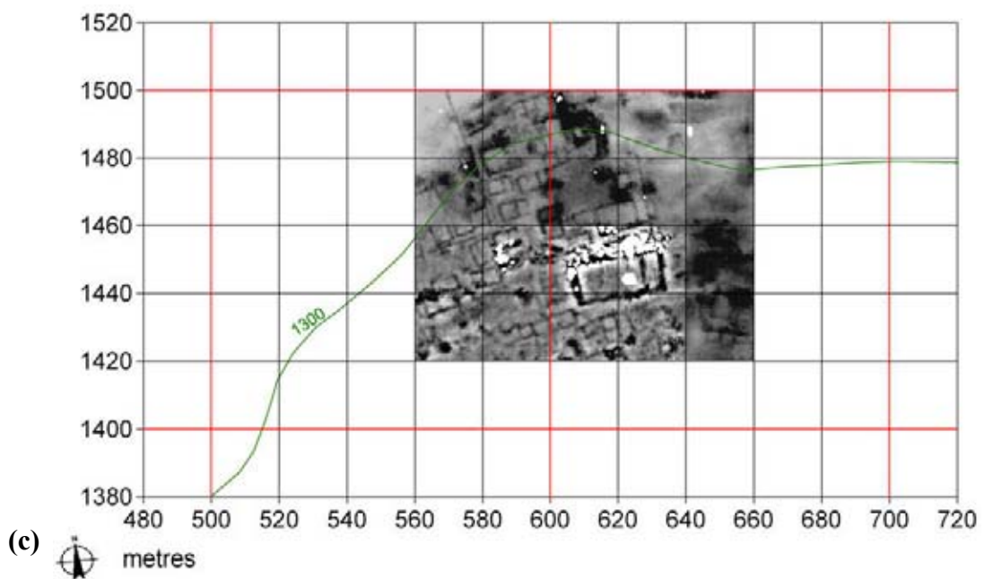
Figure 57. Maps of the Temple Area on the Central Spur generated from (a) GPS, (b) gradiometer and (c) electrical resistance survey.
