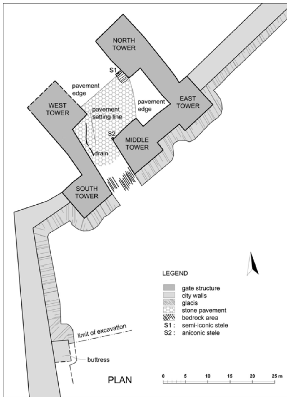
Figure 120. Plan of the Cappadocia Gate.
